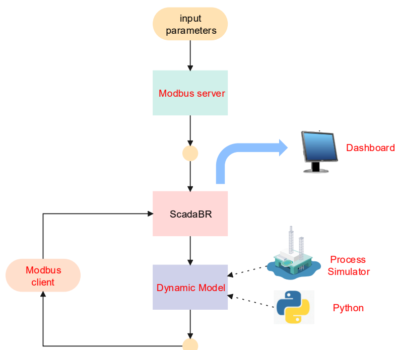
Fig.2. Simplified Flowchart of the algorithm used to link ScadaBR and Python.
