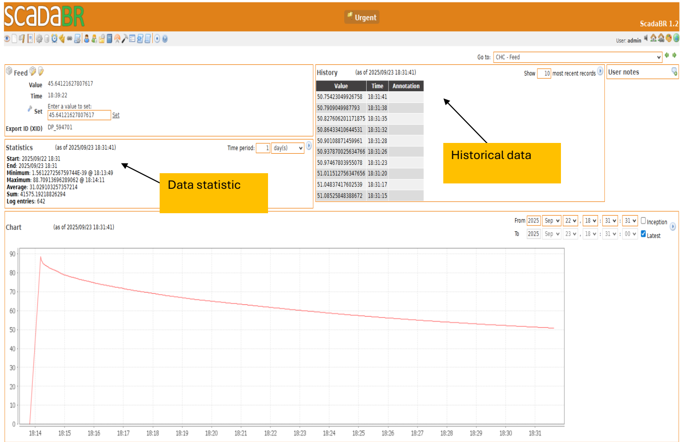
Fig. 9. Details of variable “VGO mass fraction”.
