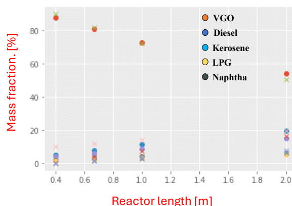
Fig.6. Model result of product's mass fraction percentages along the reactor for T = 410\text{ }^{\circ}\text{C} .
