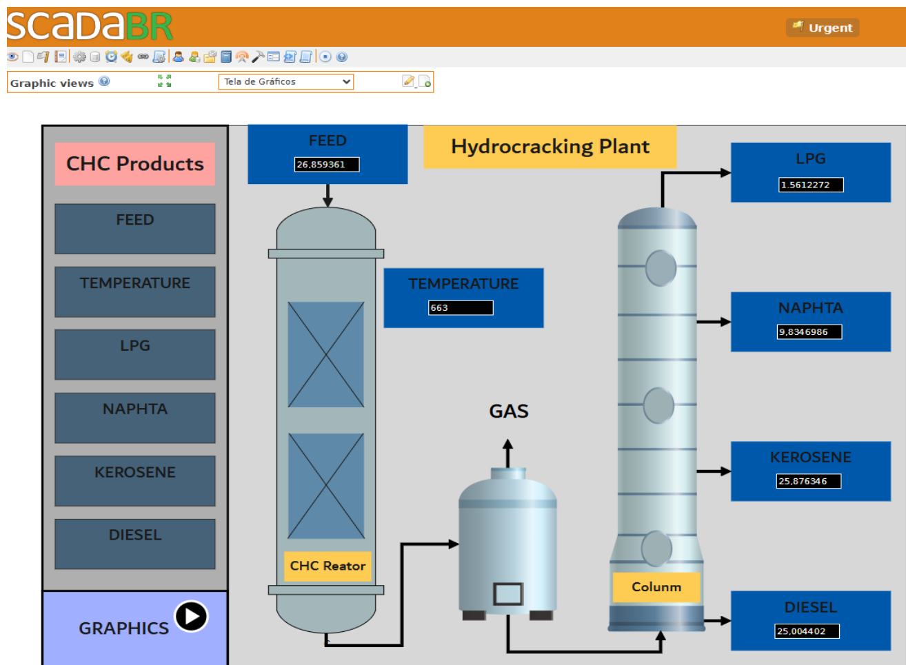
Fig. 10. CHC dashboard implemented in ScadaBR.
