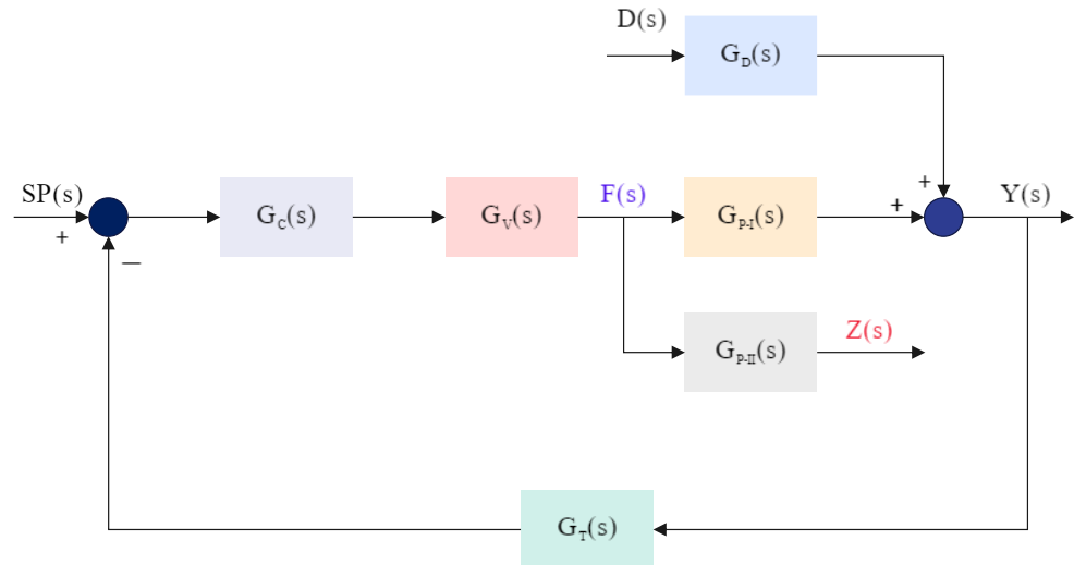
Fig.5. Representation of a feedback PID control block.
