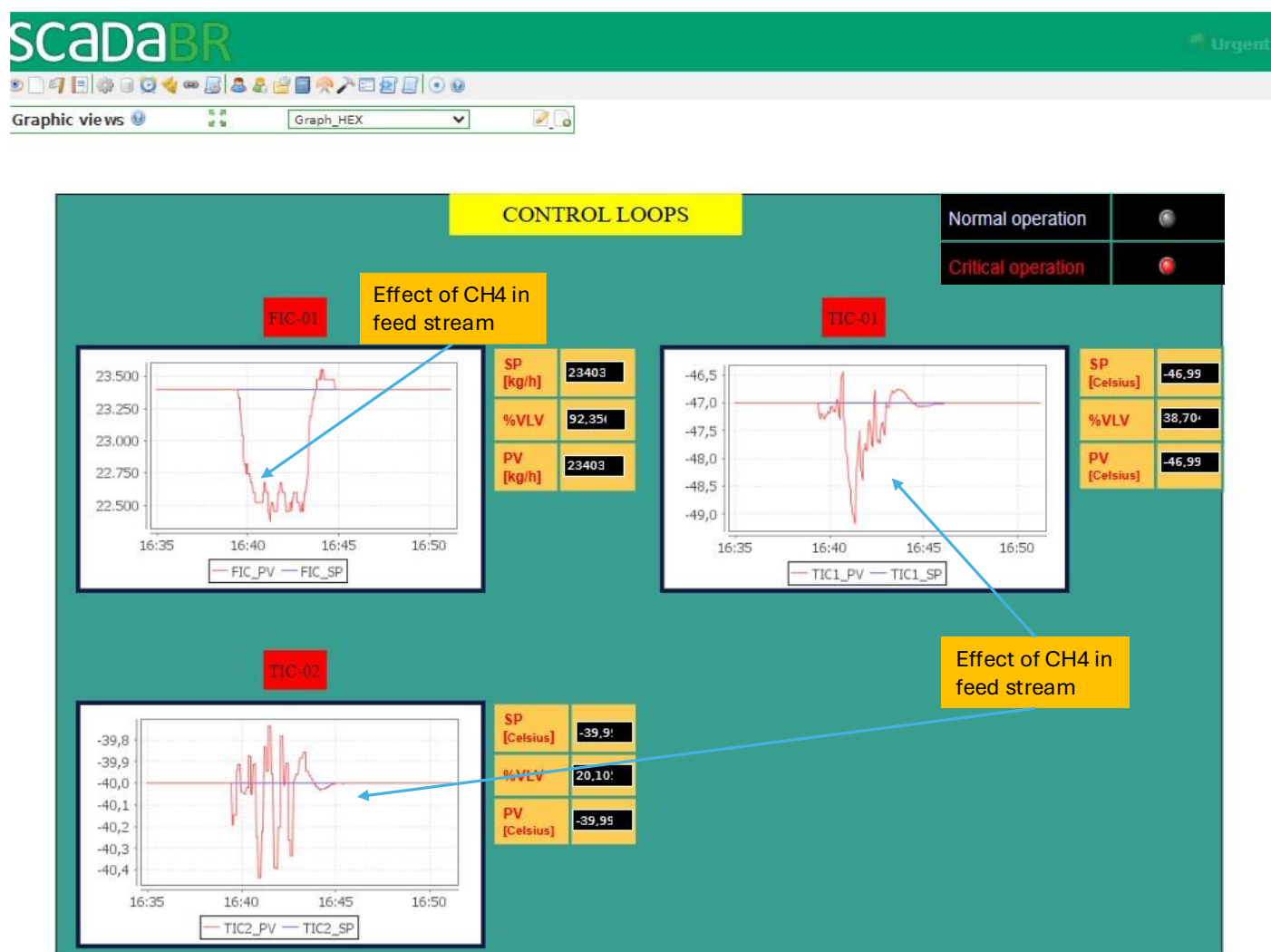
Fig. 14. Dashboard for PID Control Loops (CH 4 effects).
