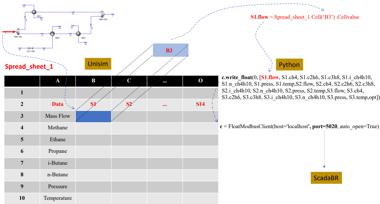
Fig. A2. Communication between Hysys-Python-ScadaBR (illustration of the Spread_sheet_1 - "Simulation").
