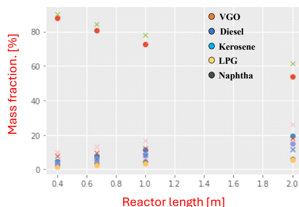
Fig.7. Model result of product's mass fraction percentages along the reactor for T = 390\text{ }^{\circ}\text{C} .
