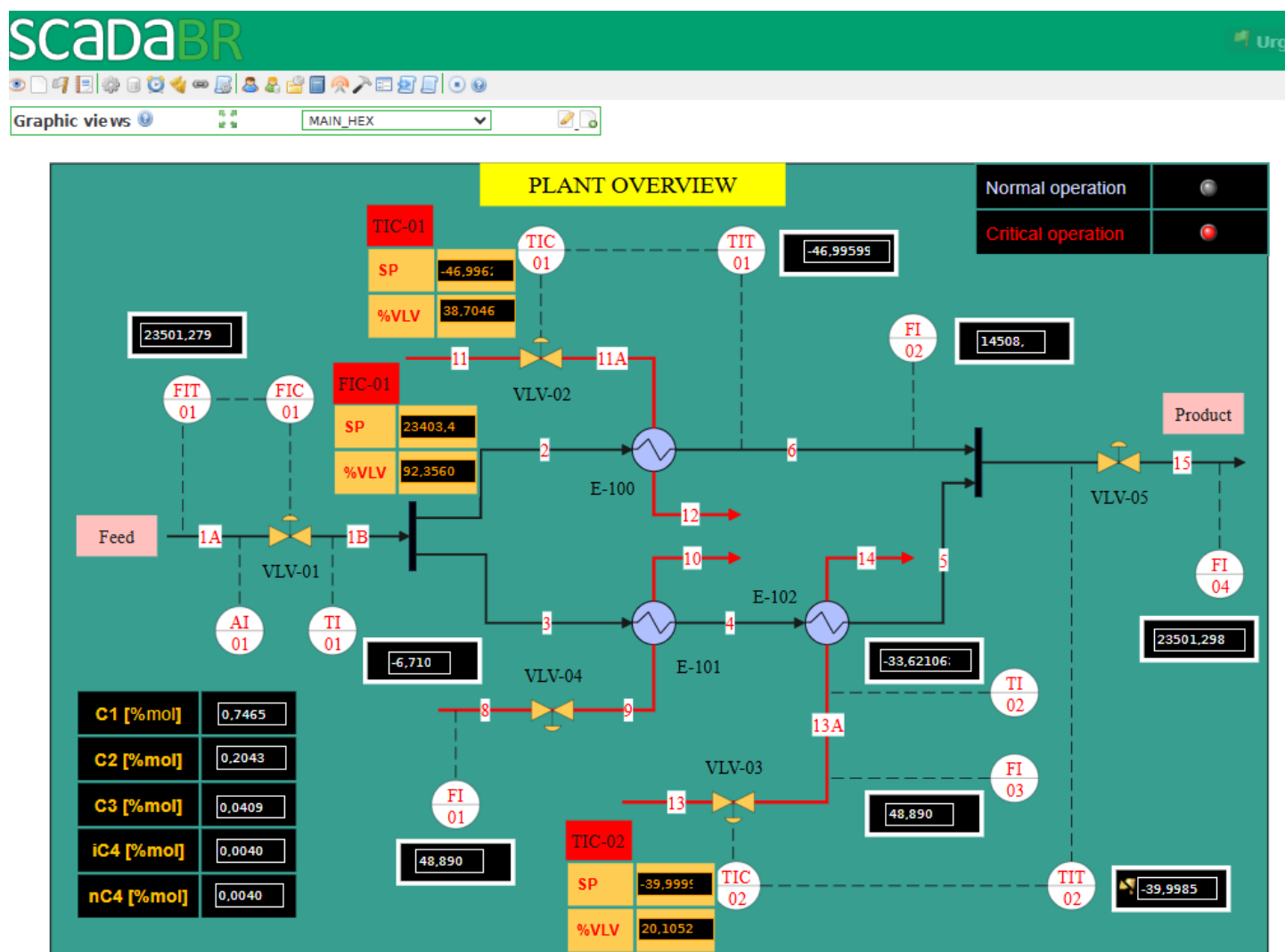
Fig. 11. Heat Exchanger Network process dashboard implemented in ScadaBR.
