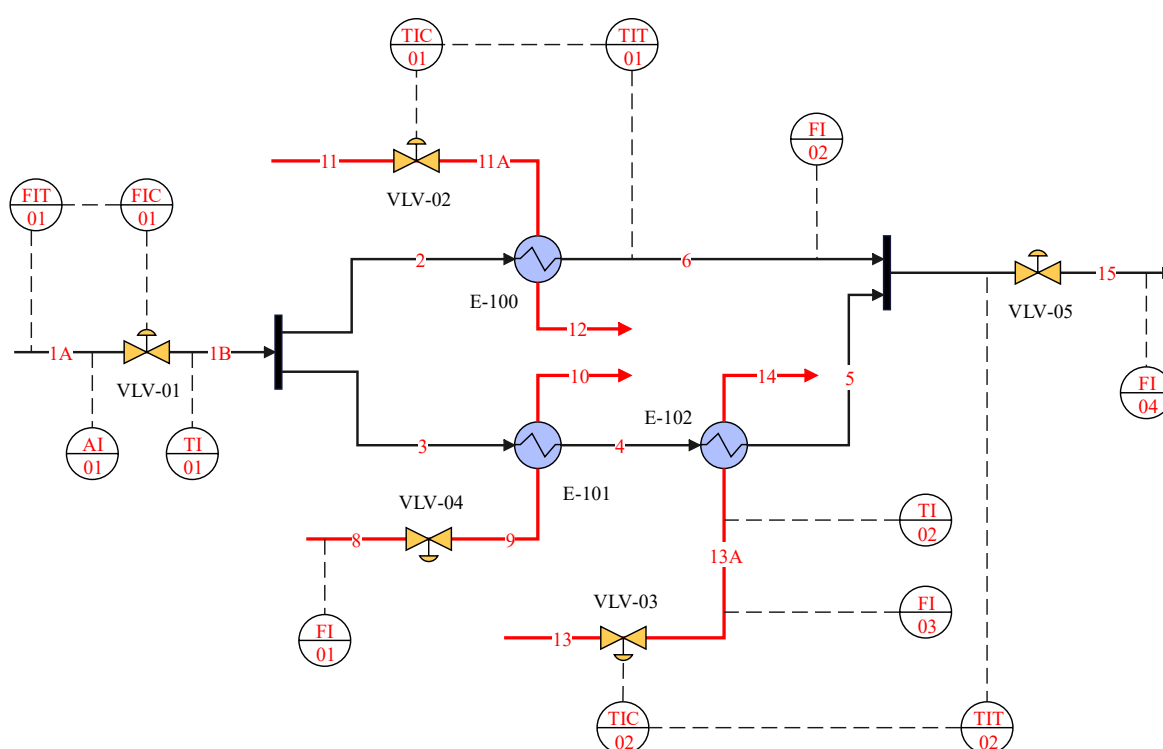
Fig.4. Hysys Flowsheet of Dynamic Simulation Applied to a Heat Exchanger Network.
