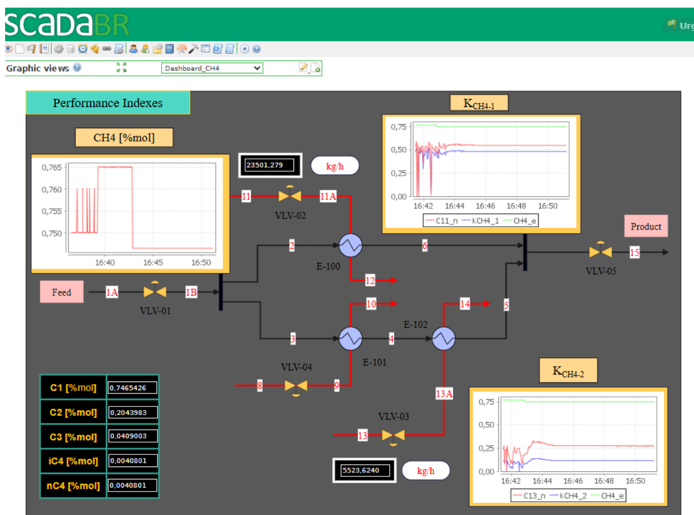
Fig. 13. Dashboard of Performance Indexes.
