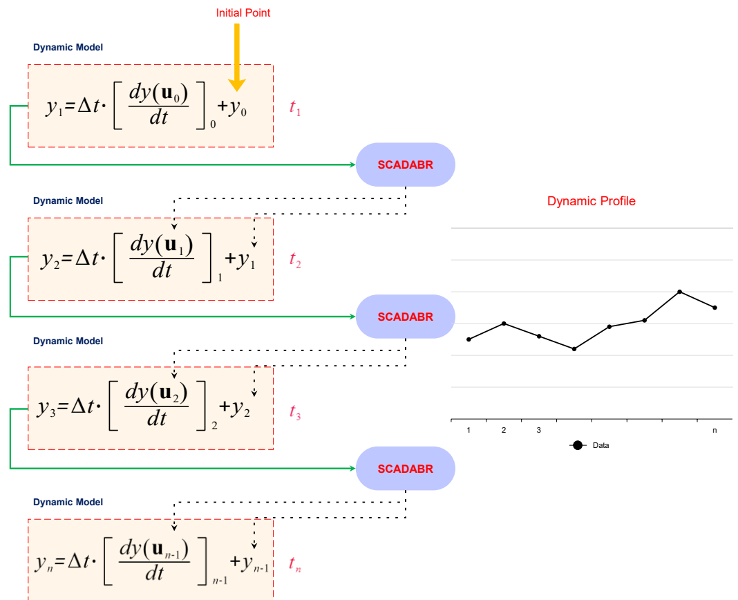
Fig.1. Simplified Flowchart of the algorithm used to link SCADABR and Python ( y : output variables; u : input variables).
