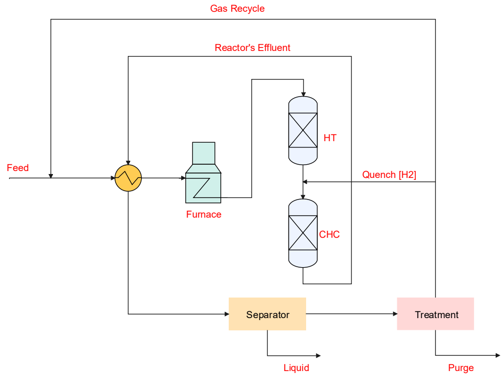
Fig.3. Hydrocracking Block Diagram [40] (HT: hydrotreating; CHC: catalytic hydrocracking).
